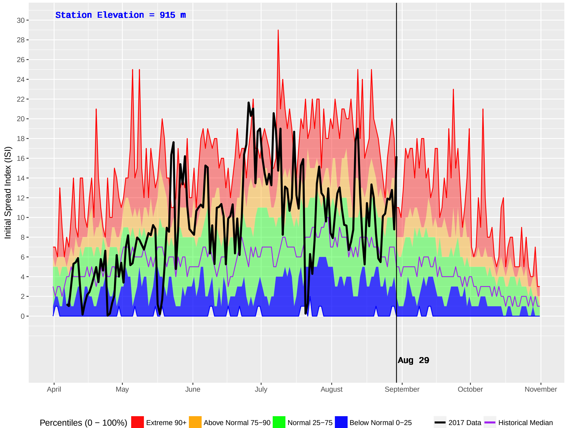
MIDDLE LAKE (226) : Historical (1989–2016) and Current (2017) Noon Initial Spread Index (ISI)
