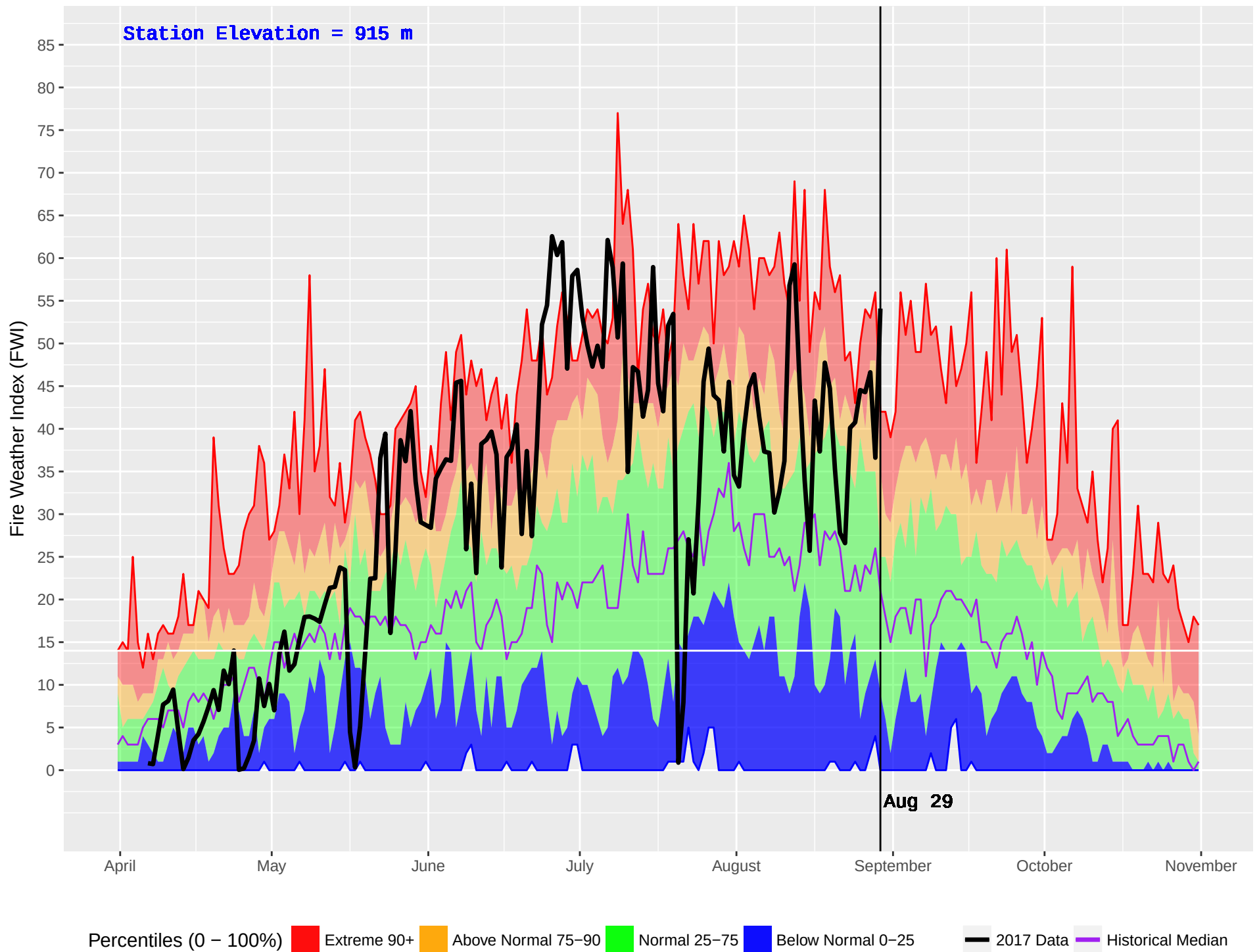
MIDDLE LAKE (226) : Historical (1989–2016) and Current (2017) Noon Fire Weather Index (FWI)
