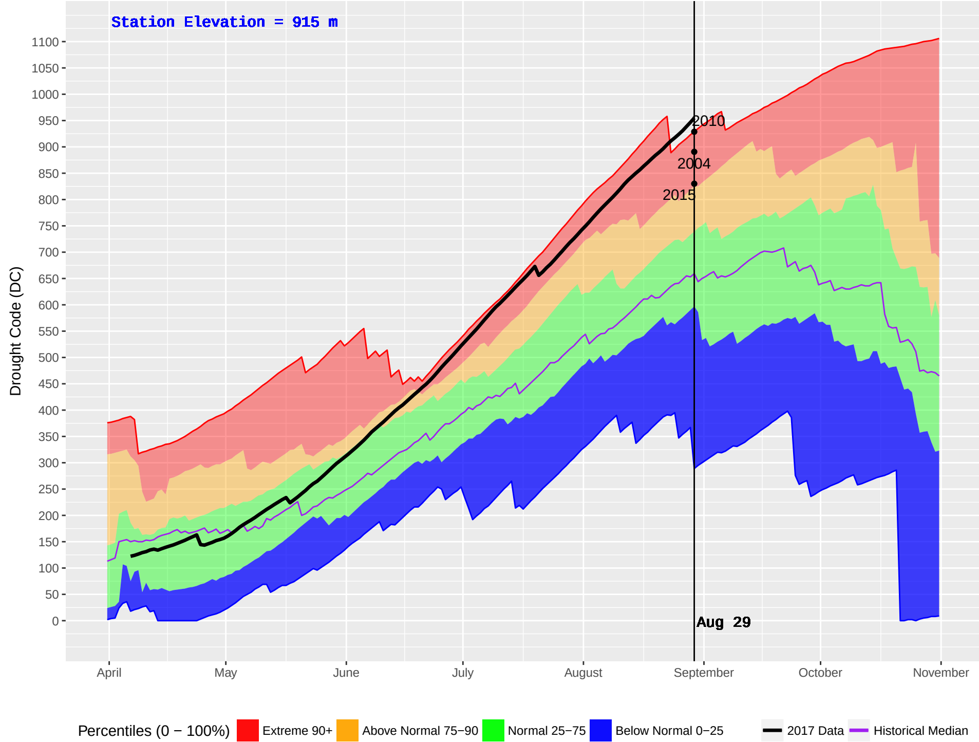
MIDDLE LAKE (226) : Historical (1989–2016) and Current (2017) Noon Drought Code (DC)
