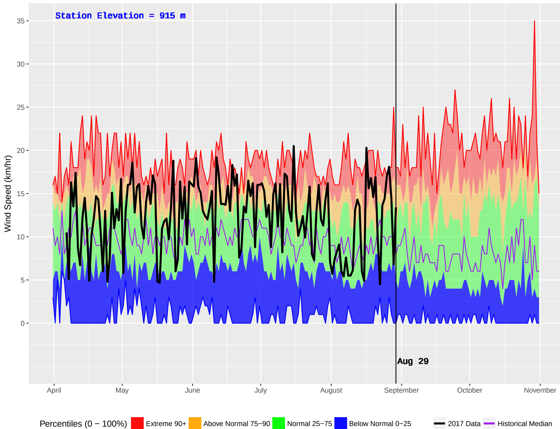
MIDDLE LAKE (226) : Historical (1989–2016) and Current (2017) Noon Wind Speed
