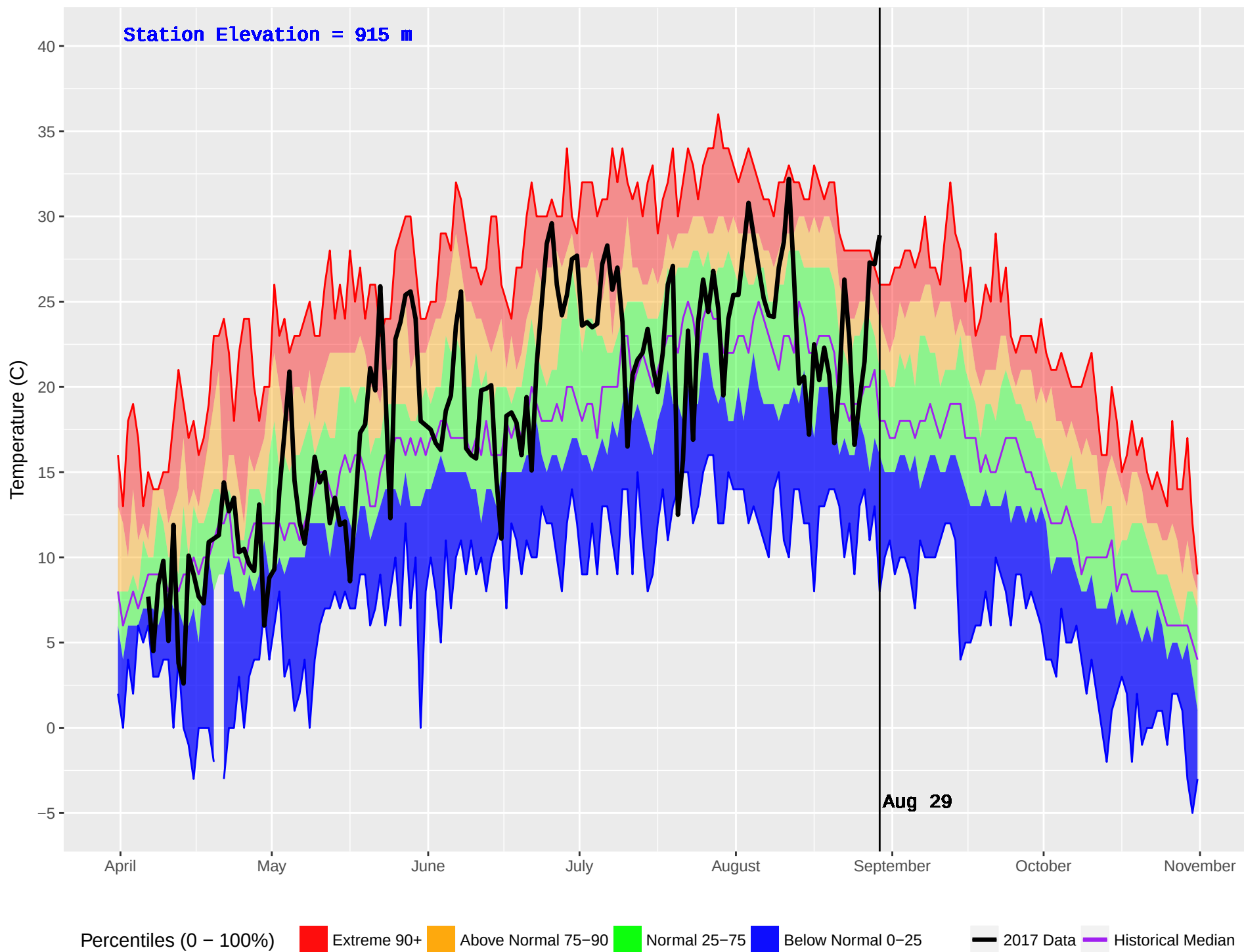
MIDDLE LAKE (226) : Historical (1989–2016) and Current (2017) Noon Temperature
