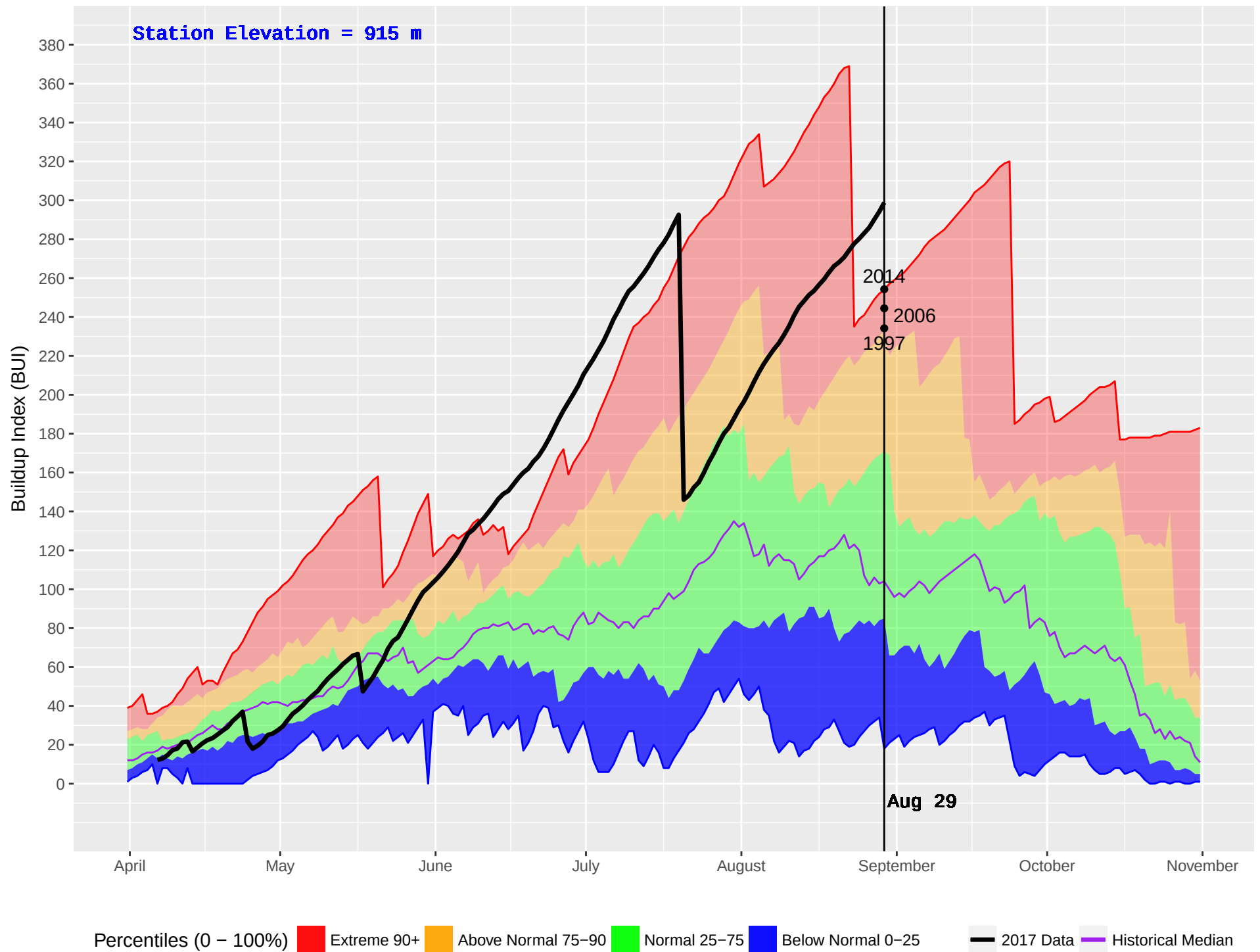
MIDDLE LAKE (226) : Historical (1989–2016) and Current (2017) Noon Buildup Index (BUI)
